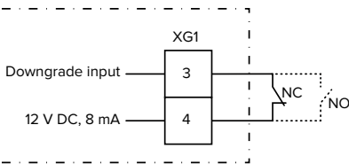
Fig. 16: Schematic circuit diagram: Connection of an external switching contact (default setting: NO)
