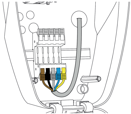
Fig. 8: Power supply connection (example)
